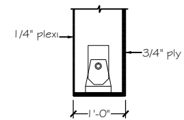
TYPICAL SECTION
